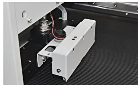
Static eliminator (UV special) Effectively eliminate static electricity to protect the printhead and improve printing accuracy
