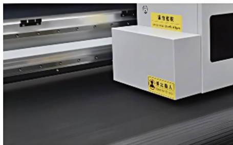
Anti collision device configured on both sides of the printhead Avoid collision between the printhead and obstacles to protect the printhead
